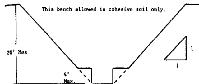
SINGLE BENCH
