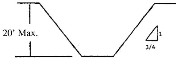
SIMPLE SLOPE – GENERAL
