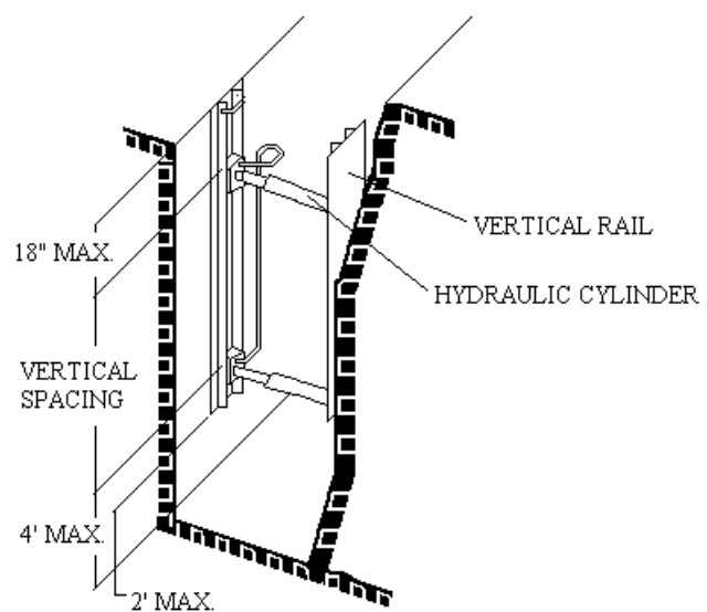
Figure 1. Aluminum Hydraulic Shoring
