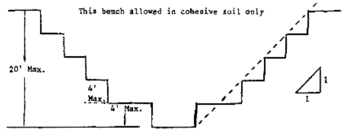
MULTIPLE BENCH
