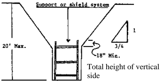
SUPPORTED OR SHIELDED VERTICALLY SIDED LOWER PORTION
