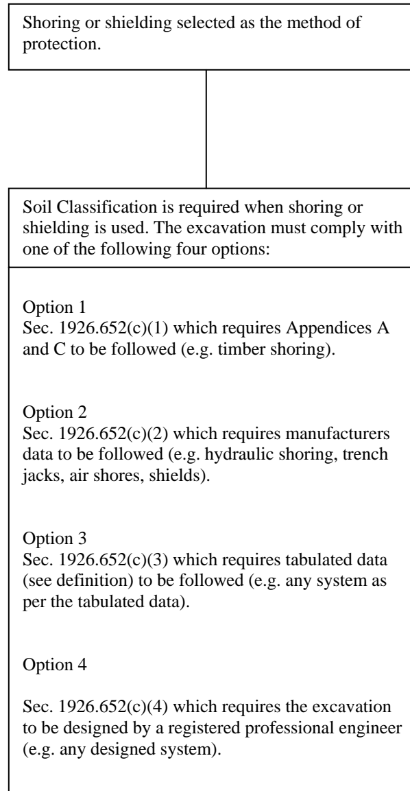
FIGURE 3 - SHORING AND SHIELDING OPTIONS
