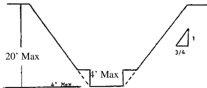
SIMPLE BENCH
