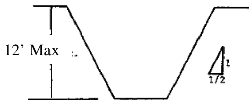
SIMPLE SLOPE - SHORT TERM
